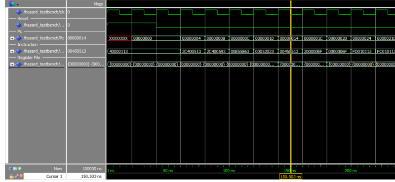
Figure 5.1: R32ICore Initialization
